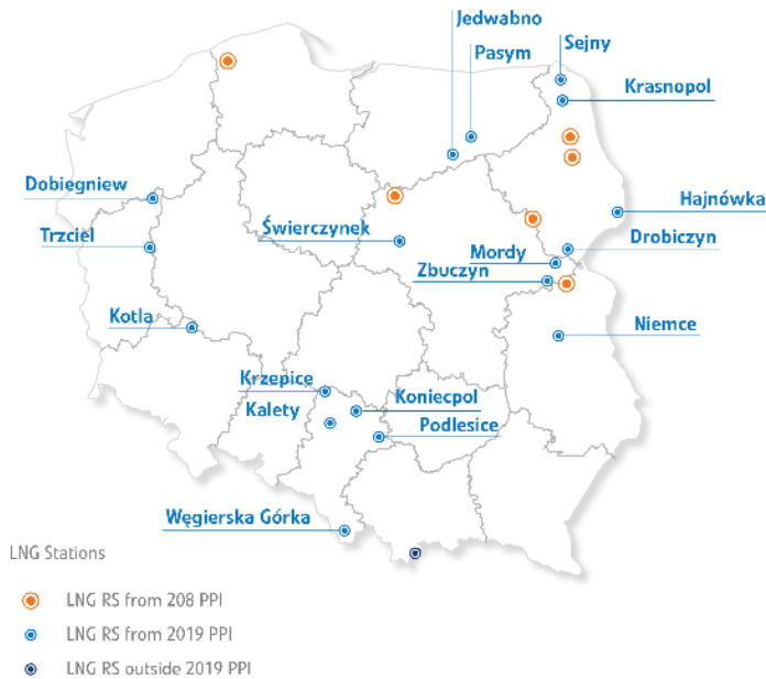
Figure 8 LNG regasification stations in Poland
